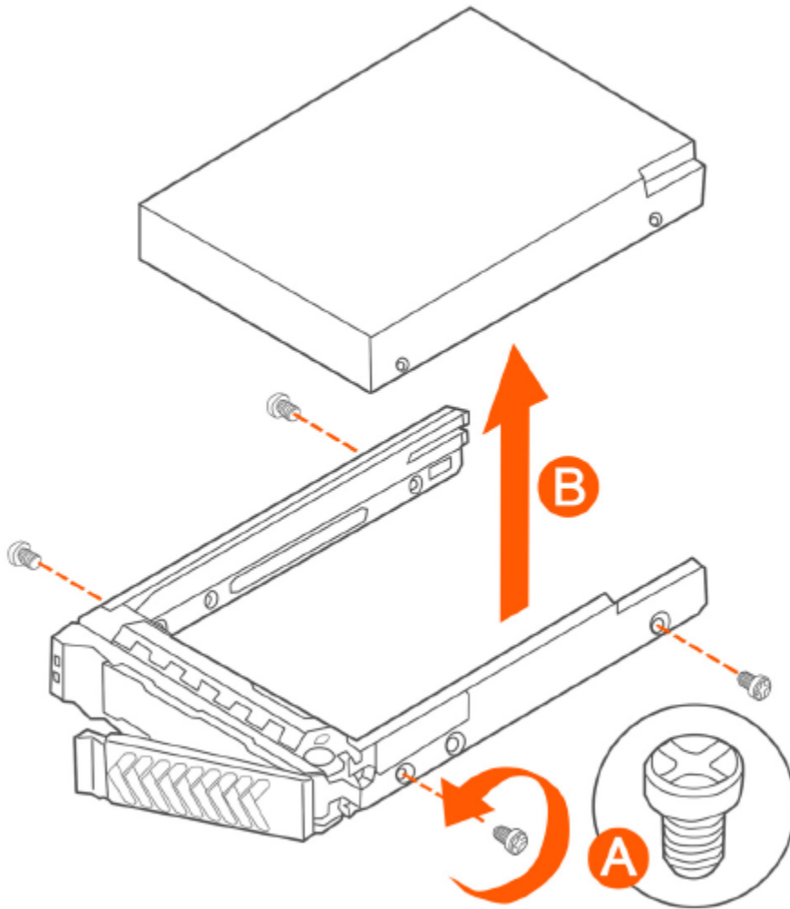
FIGURE 267 Removing the hard drive
